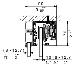
Ceiling mounting with a fixed glass profile.
