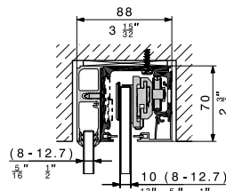
Integrated ceiling mounting with a fixed glass profile.
