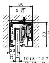
Integrated ceiling mounting without fixed glass.
