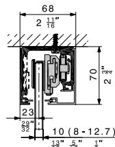
Ceiling mounting without fixed glass.
